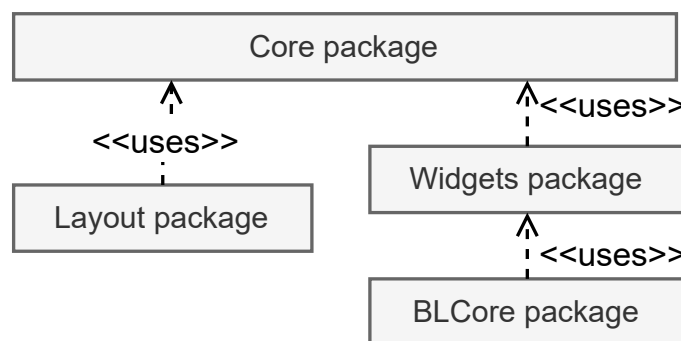
Figure 5.1: BLCore - GUI meta-model
