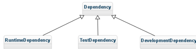
Figure 4. Dependency scopes
