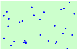
Figure 1.6: A BouncingAtomsMorph.
