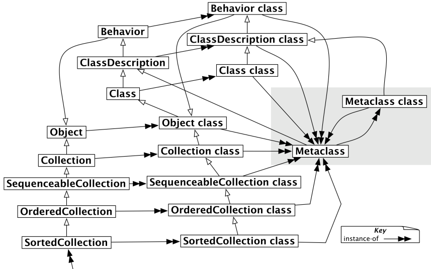
Figure 14-9 All metaclasses are instances of the class MetaClass, even the metaclass of MetaClass.
