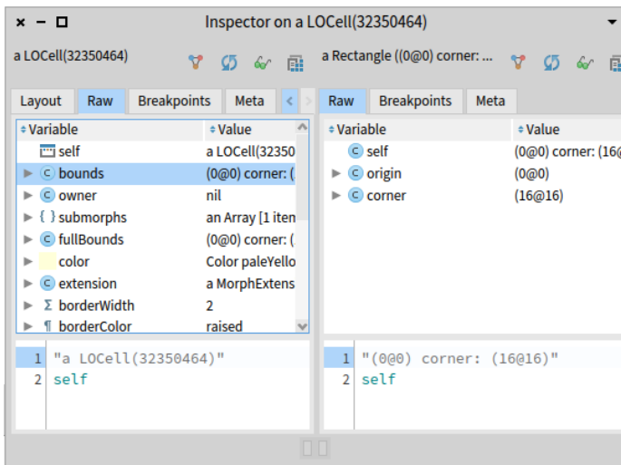
Figure 4-9 When we click on an instance variable, we inspect its value (another object).
