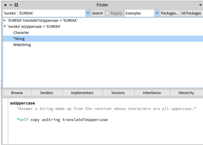
Figure 2-15 Looking for a method that given the string 'eureka' returns the string 'EUREKA'.
