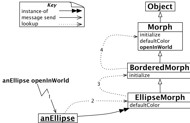
Figure 8-11 Method lookup follows the inheritance hierarchy.
