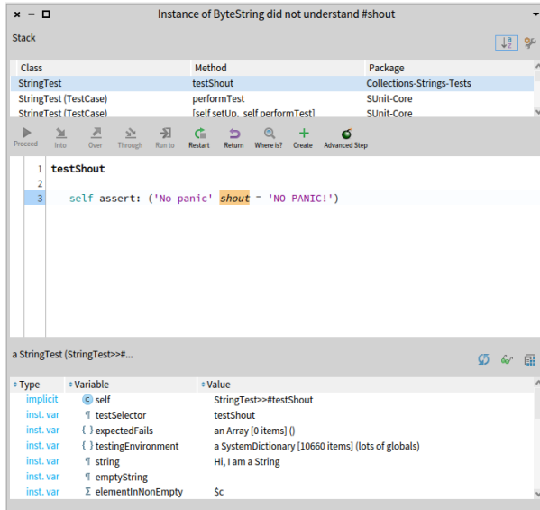
Figure 2-17 Looking at the error in the debugger.
