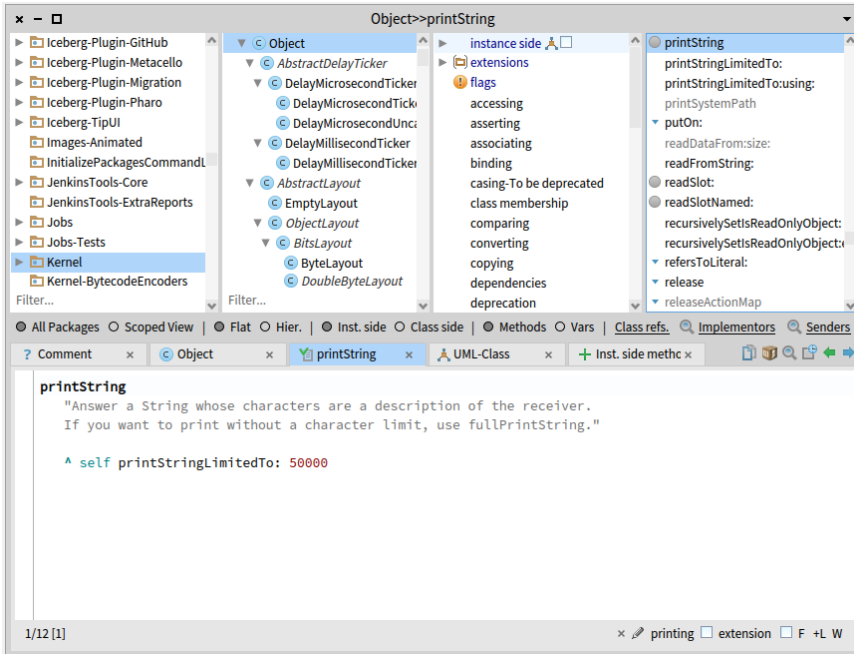
Figure 2-11 The System Browser showing the printString method of class Object .
