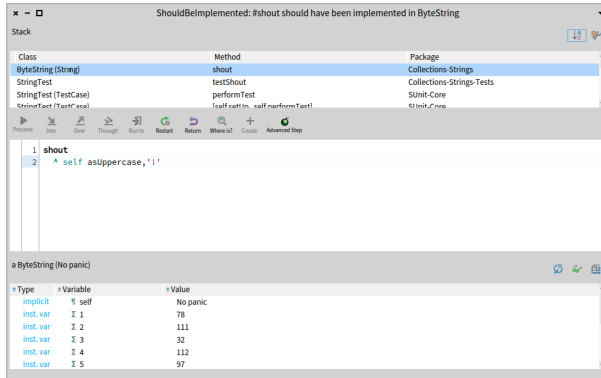
Figure 2-20 Defining the shout method right inside the debugger.
