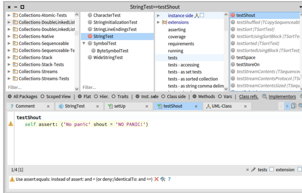
Figure 2-16 Defining a test method in the class StringTest .
