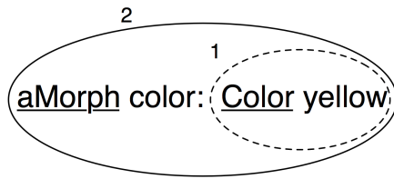
Figure 7-2 Two messages: Color yellow and aMorph color: Color yellow.
