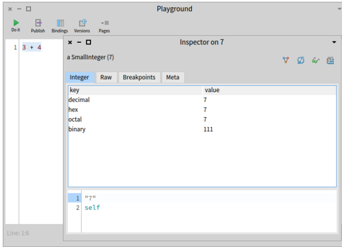
Figure 2-8 Inspecting a simple number using Inspect.
