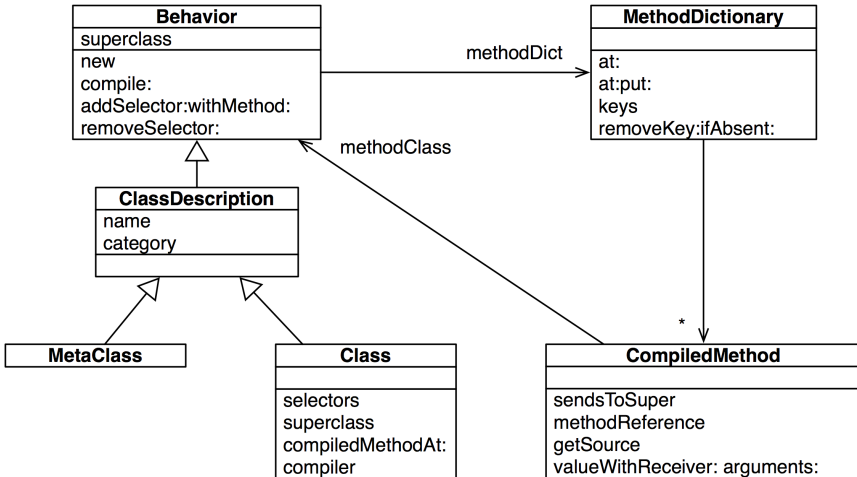
Figure 15-5 Classes, method dictionaries, and compiled methods
