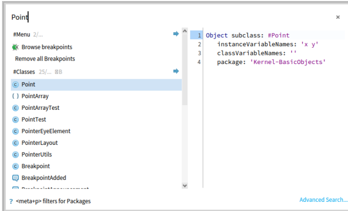
Figure 2-12 Using Spotter (shift+enter) to browse the class Point.
