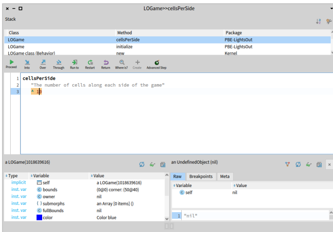
Figure 4-16 Defining cellsPerSide in the debugger.
