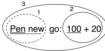
Figure 7-5 Decomposing Pen new go: 100 + 20.
