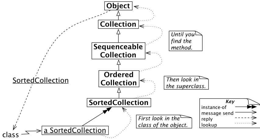
Figure 14-1 Sending the message class to a sorted collection
