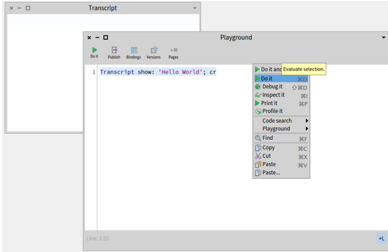
Figure 2-7 Executing an expression: displaying a string in the Transcript.
