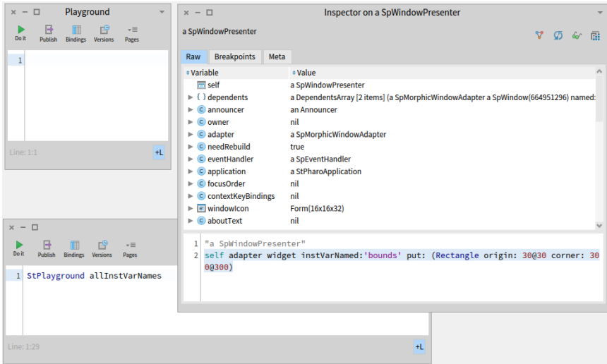
Figure 15-2 Inspecting a STPlayground.
