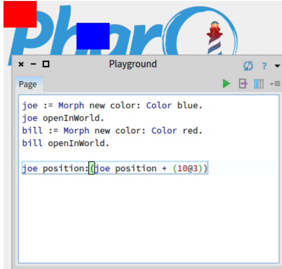
Figure 13-5 Bill and Joe after 10 moves.
