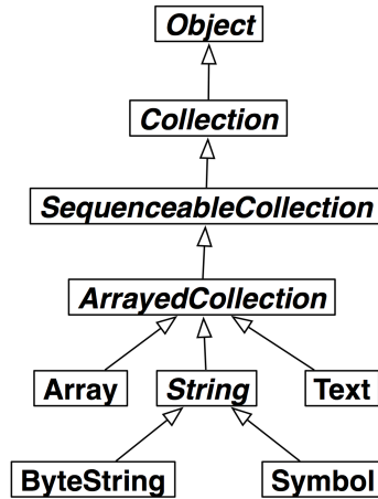
Figure 10-12 The String Hierarchy.
