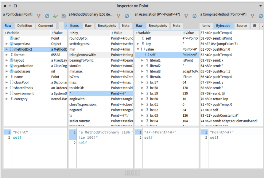
Figure 15-4 Inspector on class Point and the bytecode of its #* method.
