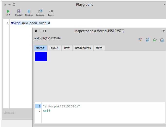
Figure 2-9 Inspecting a Morph using Inspect.
