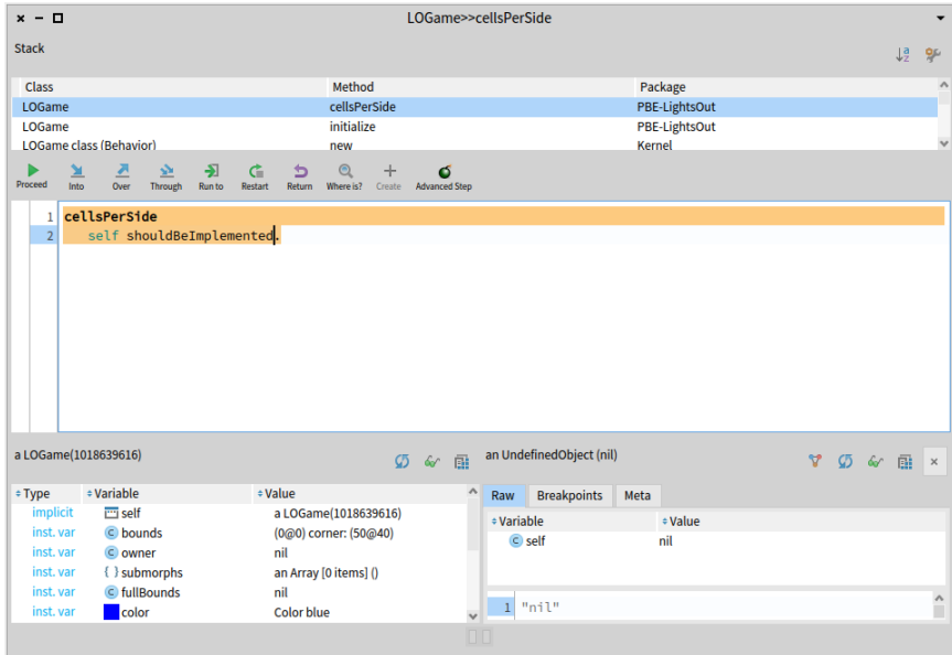
Figure 4-15 The system created a new method with a body to be defined.
