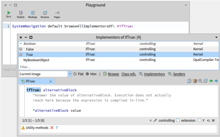
Figure 15-3 Browse all implementations of ifTrue:.
