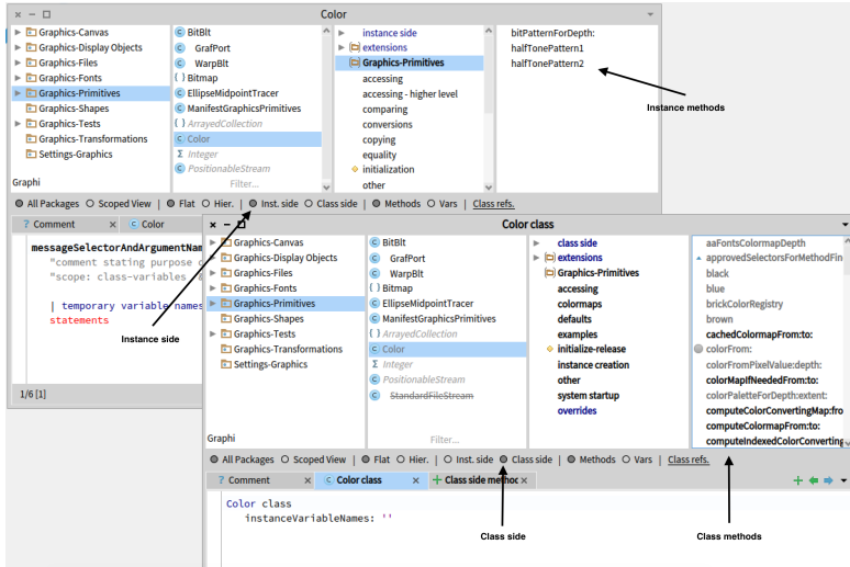
Figure 8-20 Browsing a class and its metaclass.
