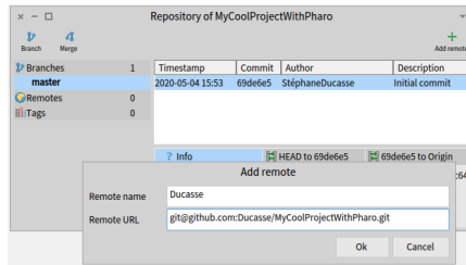
Figure 5-21 Adding a remote using the Repository browser of your project (SSH version).
