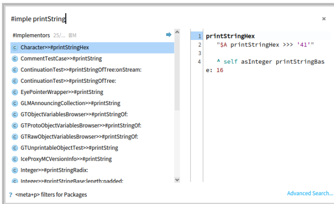
Figure 2-13 Looking for implementors matching printString.
