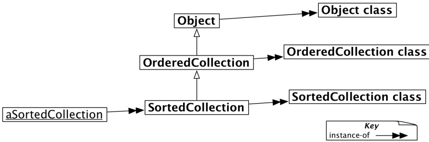
Figure 14-2 The metaclasses of SortedCollection and its superclasses (elided).
