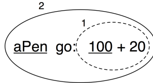
Figure 7-4 Binary messages are sent before keyword messages.
