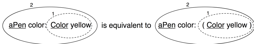
Figure 7-3 Unary messages are sent first so Color yellow is sent. This returns a color object which is passed as argument of the message aPen color:.
