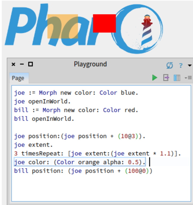
Figure 13-6 Bill follows Joe.
