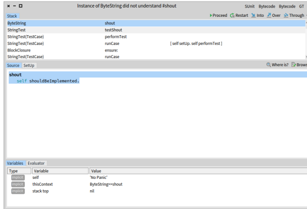
Figure 2-19 The automatically created shout method waiting for a real definition.
