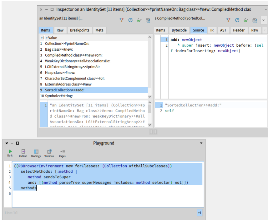
Figure 15-6 Finding methods that send a different super message.
