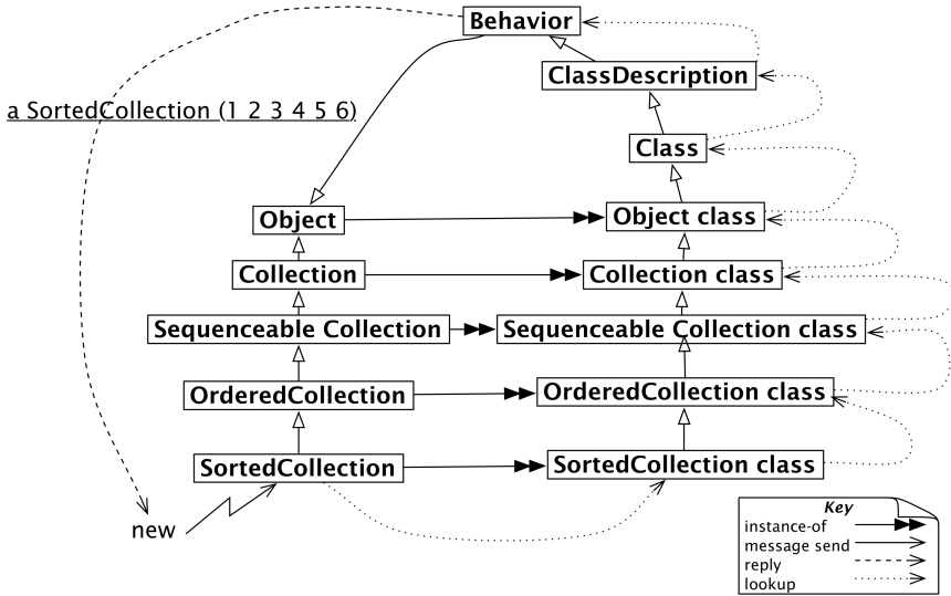
Figure 14-7 new is an ordinary message looked up in the metaclass chain.
