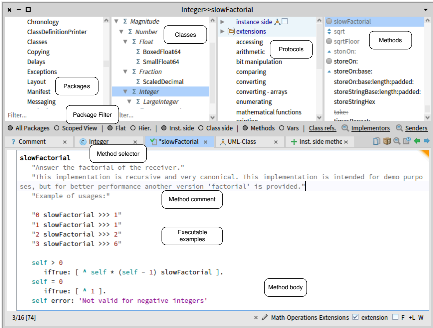
Figure 2-10 The System Browser showing the slowFactorial method of class Integer .
