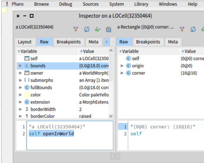
Figure 4-10 A LOMCell opened in the World.
