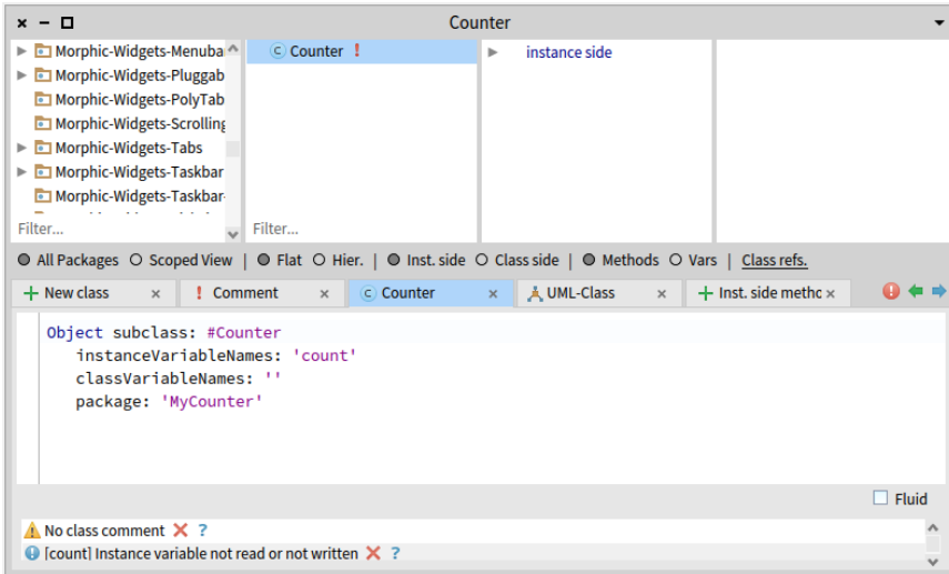
Figure 3-1 Package created and class creation template.
