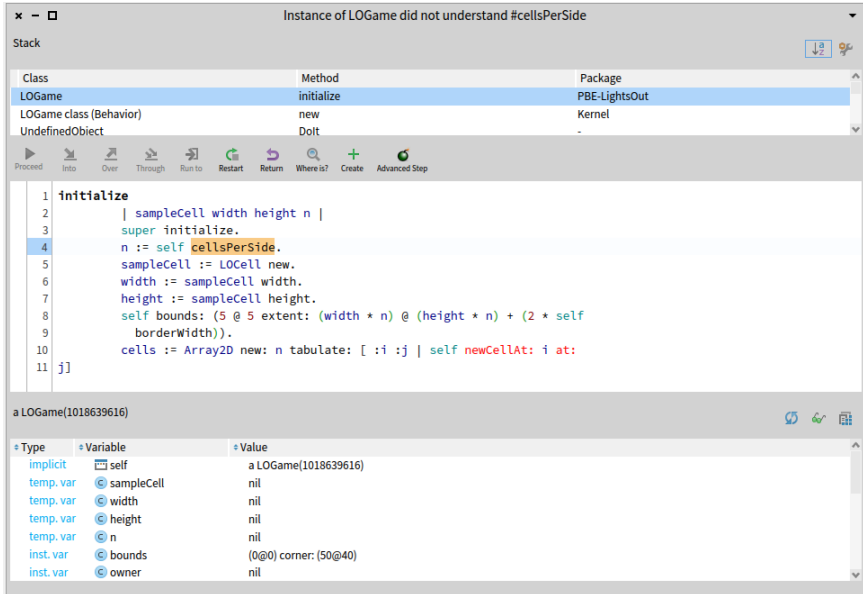
Figure 4-14 Pharo detecting an unknown selector.
