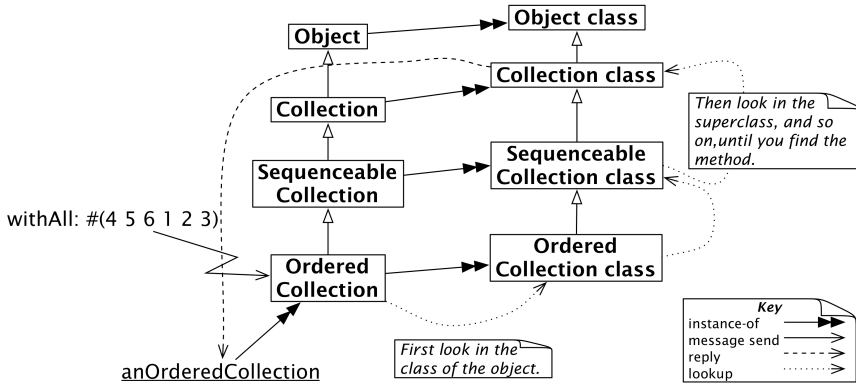
Figure 14-4 Message lookup for classes is the same as for ordinary objects.
