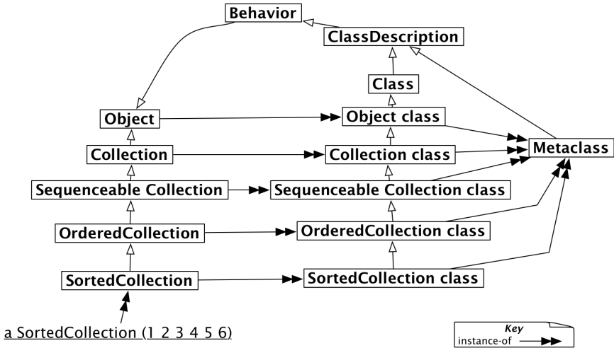
Figure 14-8 Every metaclass is a MetaClass.
