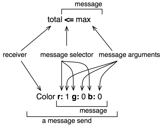
Figure 7-1 Two message sends composed of a receiver, a method selector, and a set of arguments.
