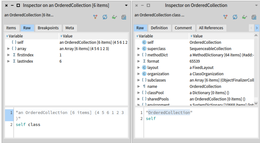
Figure 14-5 Classes are objects too.
