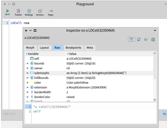
Figure 4-8 The inspector used to examine a LOCell object.
