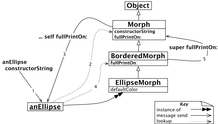
Figure 8-19 self and super sends.
