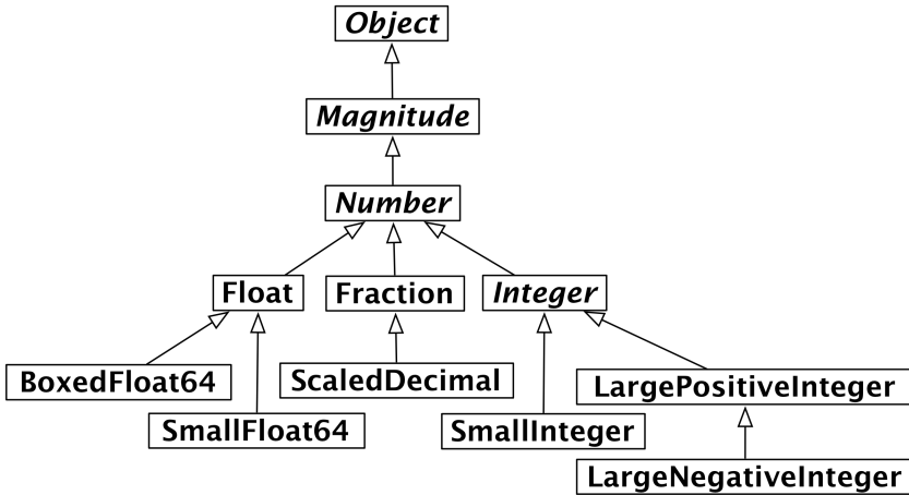
Figure 10-10 The number hierarchy.
