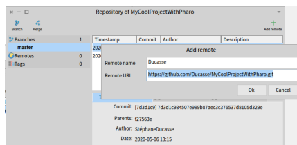
Figure 5-22 Adding a remote using the Repository browser of your project (HTTP version).
