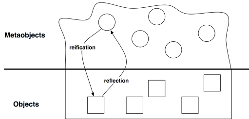
Figure 15-1 Reification and reflection.
