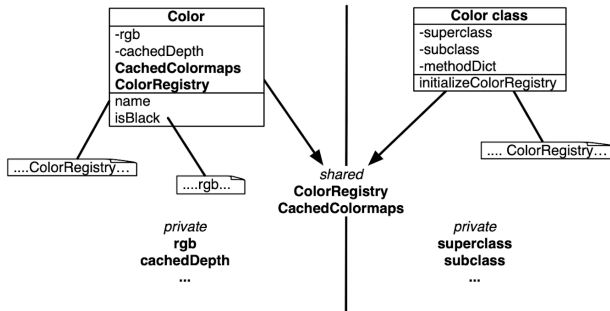
Figure 8-33 Instance and class methods accessing different variables.
