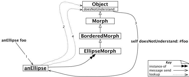
Figure 8-13 Message foo is not understood.
