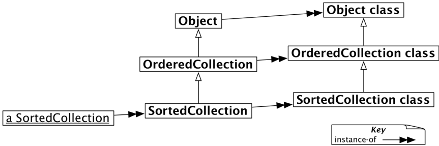
Figure 14-3 The metaclass hierarchy parallels the class hierarchy (elided).
