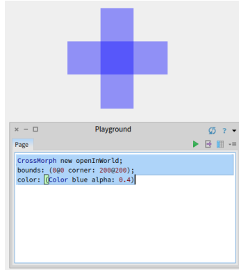
Figure 13-9 The center of the cross is filled twice with the color.
