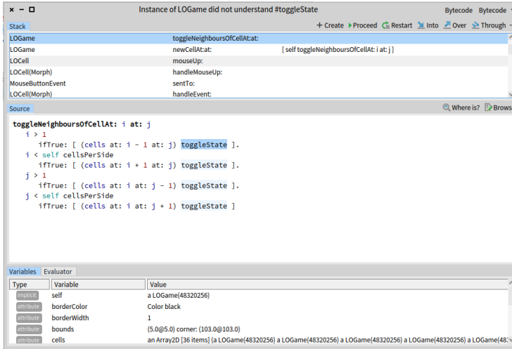
Figure 4-22 The debugger, with the method toggleNeighboursOfCellAt:at: selected.
