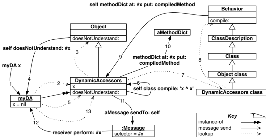
Figure 15-8 Dynamically creating accessors.
