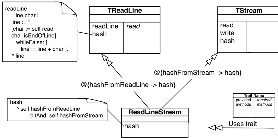
Fig. 1. The class ReadLineStream implements a stream that read lines by using two traits TReadLine and TStream.
