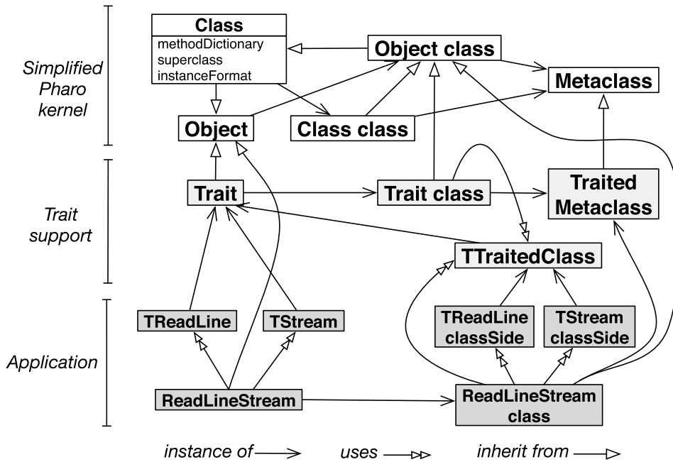
Fig. 5. The final model of our implementation, including the TTraitedClass trait. This trait provides the required behaviour to handle traits to the classes using traits.
