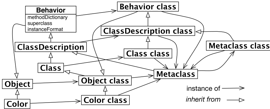
Fig. 2. Initial and traditional Pharo kernel (without traits). The class kernel is decomposed in Behavior (root of all metaclasses and classes), ClassDescription, and Class and Metaclass. Behavior defines the essence of a class (superclass, a method dictionary and a way to describe instance state [5]).
