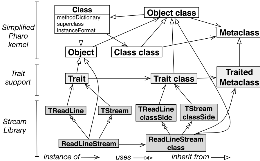
Fig. 4. The traits TStream and TReadLine are instances of Trait, their class-side counter parts, TStream classSide and TReadLine classSide are instances of the class Trait class. The class ReadLineStream is an instance of the class ReadLineStream class which is an instance of the new metaClass TrainedMetaClass that manages classes using traits.
