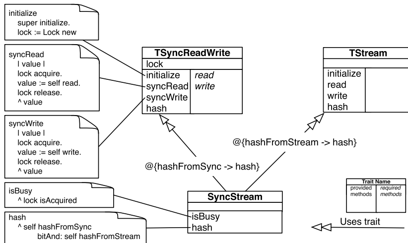
Fig. 6. The class SyncStream uses two traits TSyncReadWrite and TStream.
