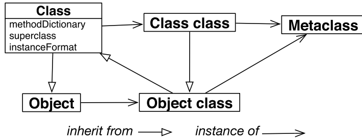
Fig. 3. Simplified traditional Pharo kernel (without traits). We compacted the Behavior, ClassDescription, Class and MetaClass in the class Class as in CLOS [24].
