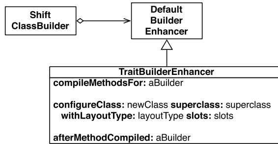
Fig. 8. The ShiftClassBuilder, used by our implementation, is extensible through pluggable build enhancers.
