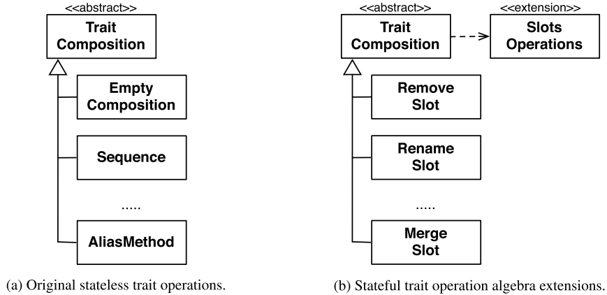
Fig. 7. Extensible trait composition algebra: the original stateless trait operations are implemented in an extensible way (a) and are extended to support stateful trait operations.
