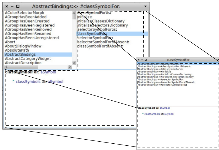
Fig. 3. The classes browser reusing the methods browser and adapting its layout.
