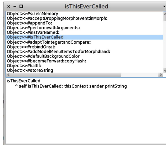
Fig. 7. The methods browser.
