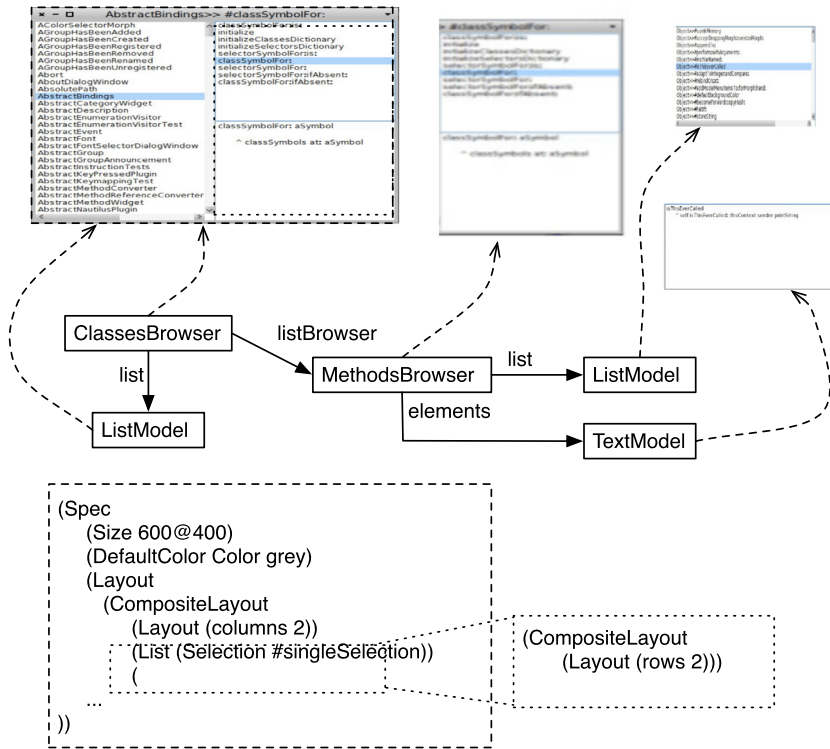
Fig. 1. Spec principles: a UI is based on a class that defines the application logic and glues visual components or other application classes together using value holders.
