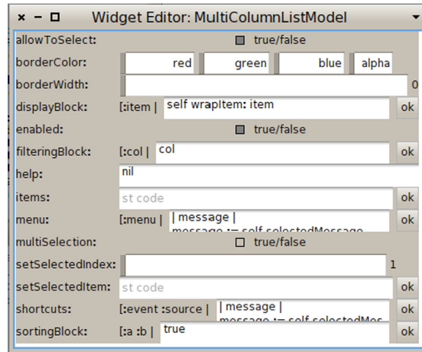
Fig. 10. Living editor on a multi columns list.
