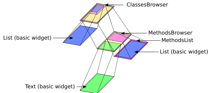
Fig. 4. A ClassesBrowser is composed of a list and a MethodBrowser. A MethodBrowser is composed of a Text and a MethodsList, which itself is composed of a List.
