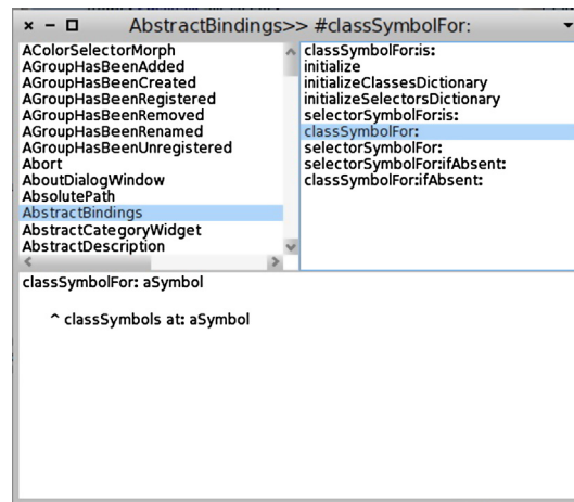
Fig. 8. The classes browser, reusing the methods browser and adapting its layout to use a classic layout.
