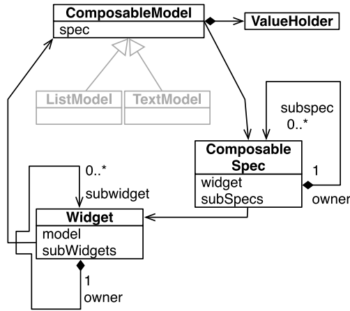
Fig. 2. Relationships between composable models, widgets and specifications.
