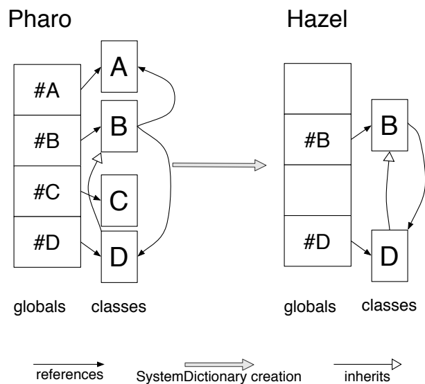
Figure 4.4: Step 3 - Reroute the remaining dependencies
