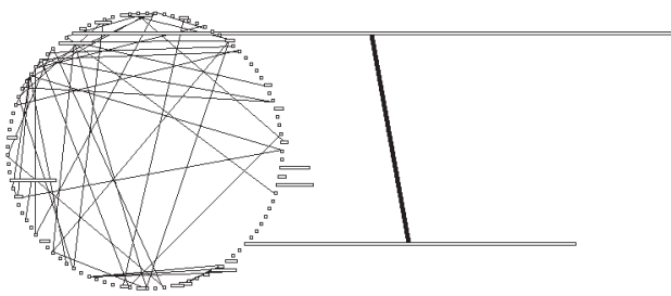
Figure 3. The Duplication Web of the MAIL-SORTING system with LIC (Lines of file-internally Copied Code) as node width.
