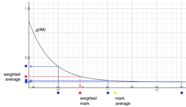
Figure 1. Computing the weighted average in Squale (here \lambda = 9 ): First, points 0.5, 1.5, and 3 (darker dots on X axis) are weighted (darker dots on Y axis), then these are averaged (lighter dot on Y axis), and this average is converted back to the [0, 3] interval (lighter dot on X axis, close to 1). The very light grey dot on X axis, past 1.5, shows the arithmetic mean of the 3 initial values
