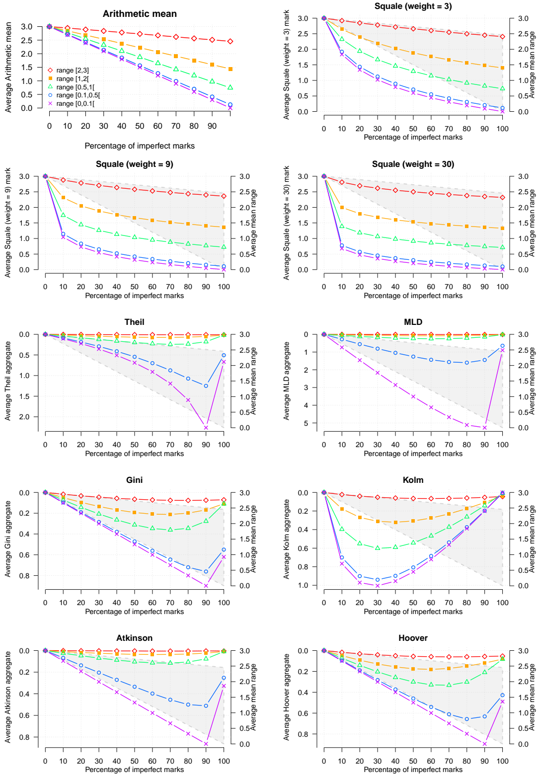
Figure 2. Results of experiments for all aggregation indexes (see text for explanation). The topmost left figure displays the common legend.
