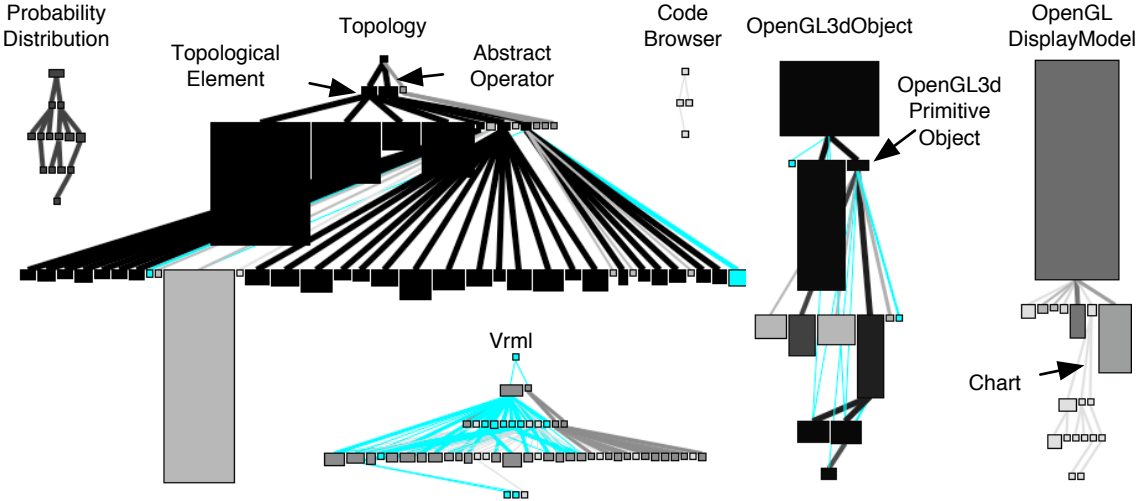
Figure 5. A Hierarchy Evolution Complexity View of the evolution of six hierarchies from the 40 versions of Jun.
