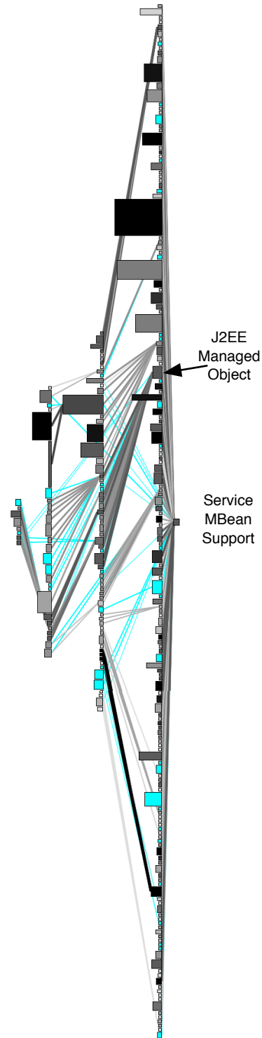
Figure 3. A Hierarchy Evolution Complexity View of the evolution of the largest hierarchy from 14 versions of JBoss.
