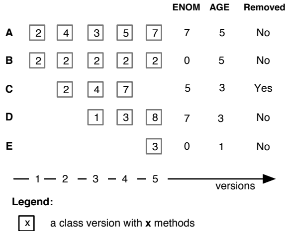
Figure 1. An example of history measurements.
