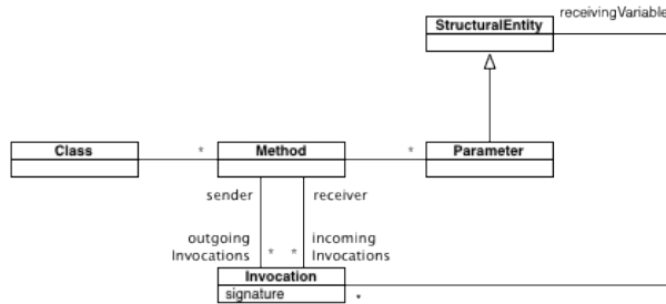
Figure 3.4: Invocations.
