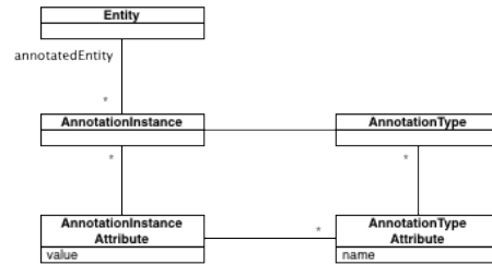
Figure 3.3: Annotations.
