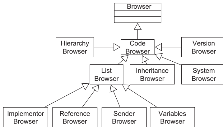
Fig. 18. Some code browsers developed using OmniBrowser framework.
