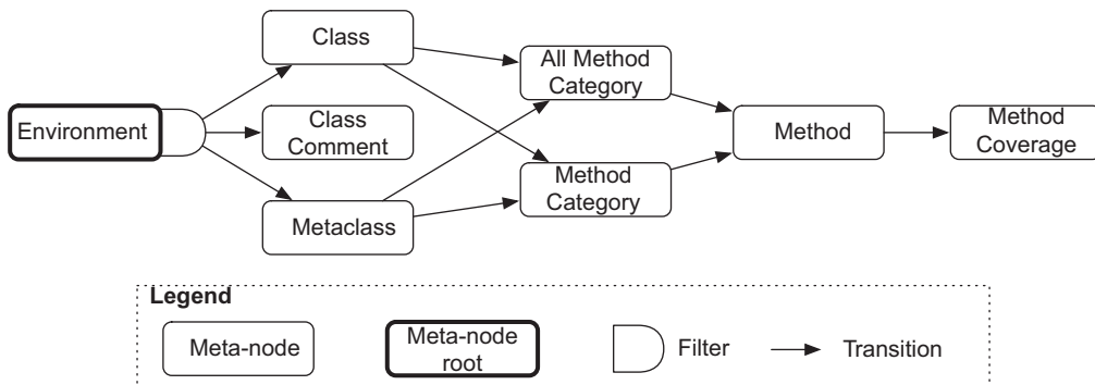
Fig. 12. Metagraph for the coverage browser.
