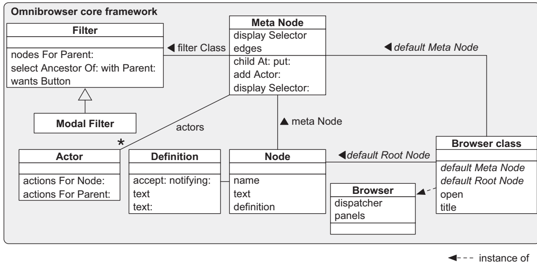
Fig. 2. Core of the Omnibrowser framework.
