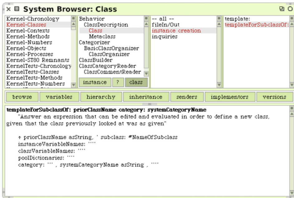
Fig. 7. OmniBrowser framework-based Smalltalk system browser.
