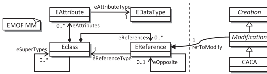
Figure 15. CACA operator metamodel.
