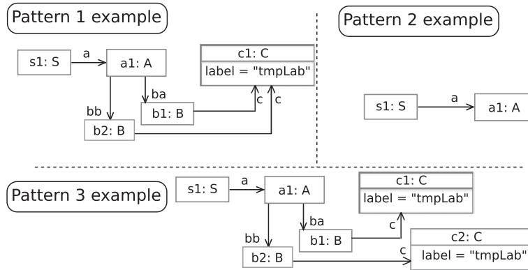
Figure 18. Patterns examples.
