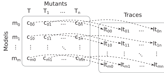
Figure 7. Mutation matrix.
