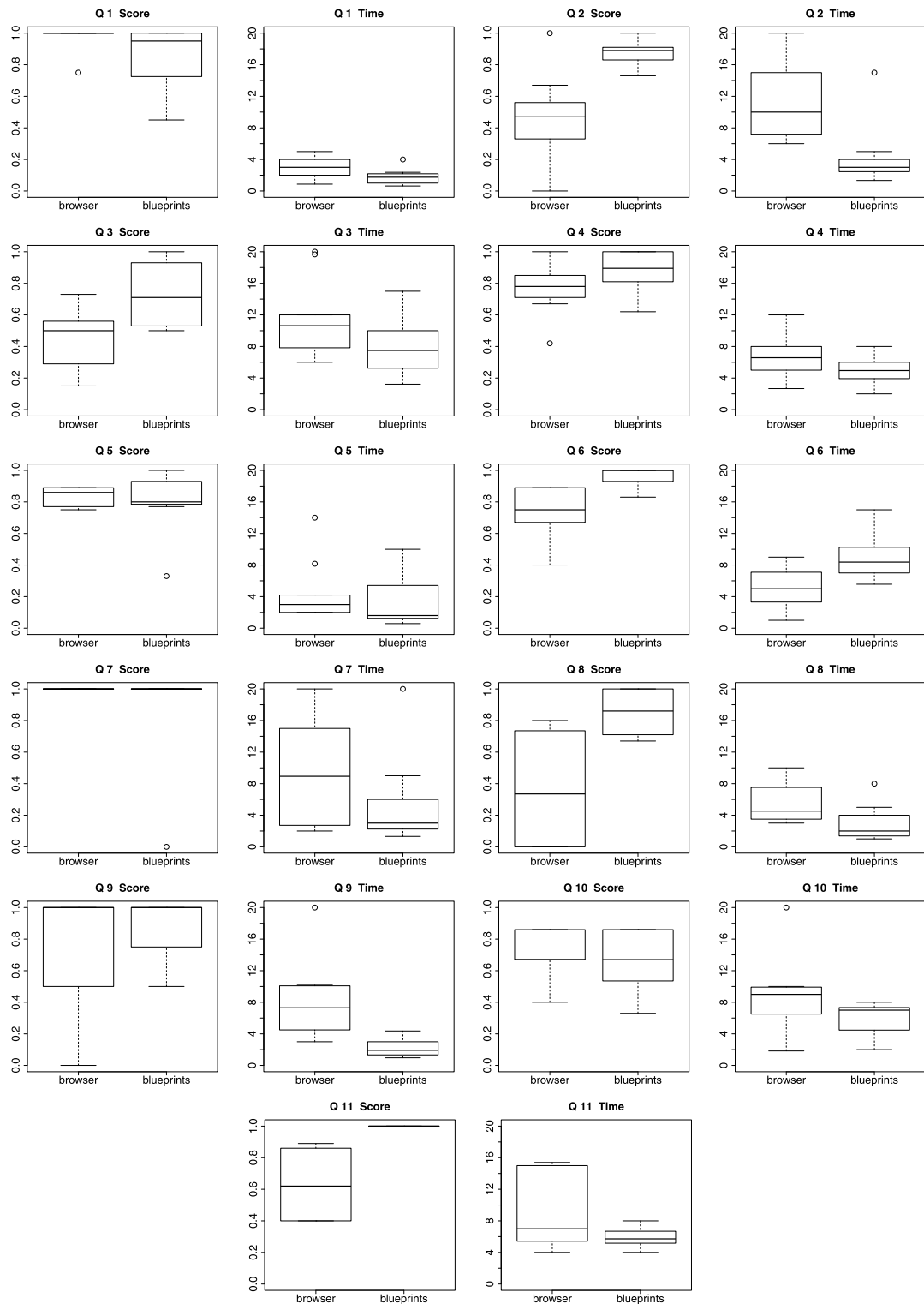
Fig. 7. Boxplots showing score and time for questions 1 to 11. Browser group shown on left and package blueprints on right for each question.
