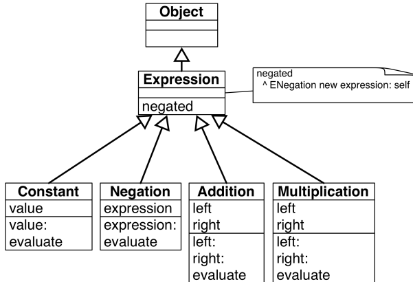
Figure 1-5 Introducing a common superclass.
